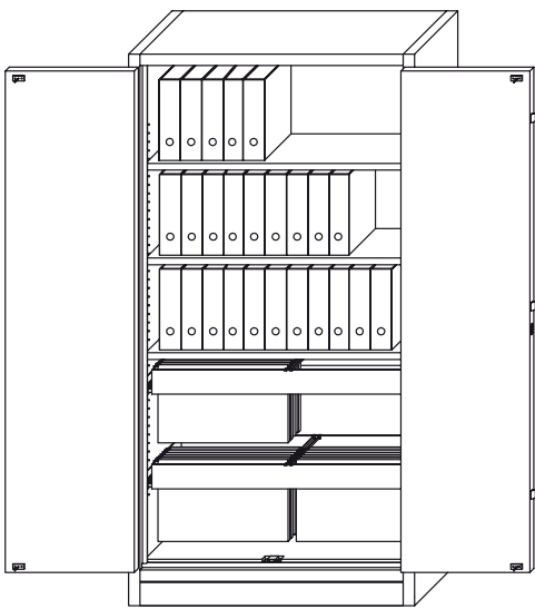
AS92:196-106-F-HRA-S 3 Shelves 2 Vertical filing drawers
