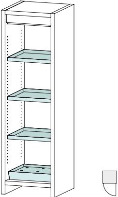
EN91-196-060 3 tank bottoms, 1 floor pan with perforated plate insert
