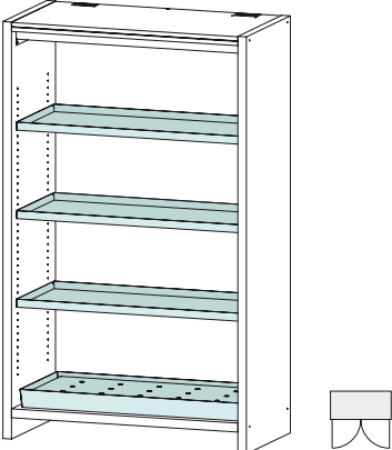
EN92:196-120 3 tank bottoms, 1 floor pan with perforated plate insert
